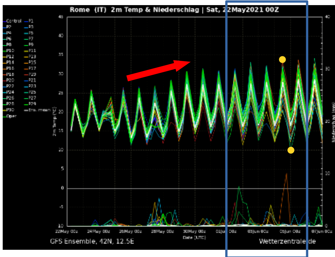
Rome, temperature e precipitation, ensemble of GFS forecast model
